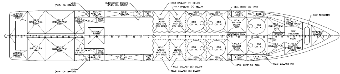
HOLD PLAN
